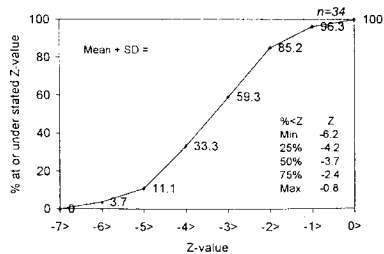
Fig. 2. Cumulative frequency distribution of preoperative Z-value
