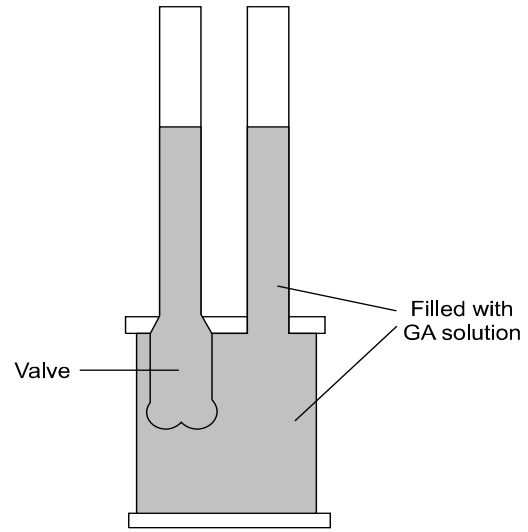
Fig. 1. Schematic view of frame for GA fixation.
